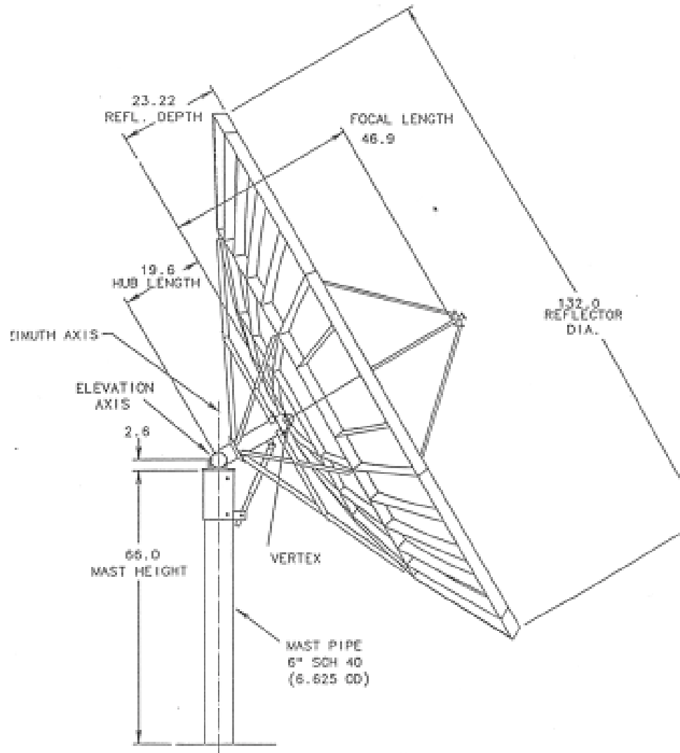
3.4 Meter Series 1344 Receive Only Axisymmetric Az/EI Antenna Geometry
